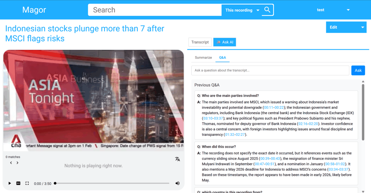
Figure 4.28: Q&A interface
